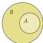
A \subset B
